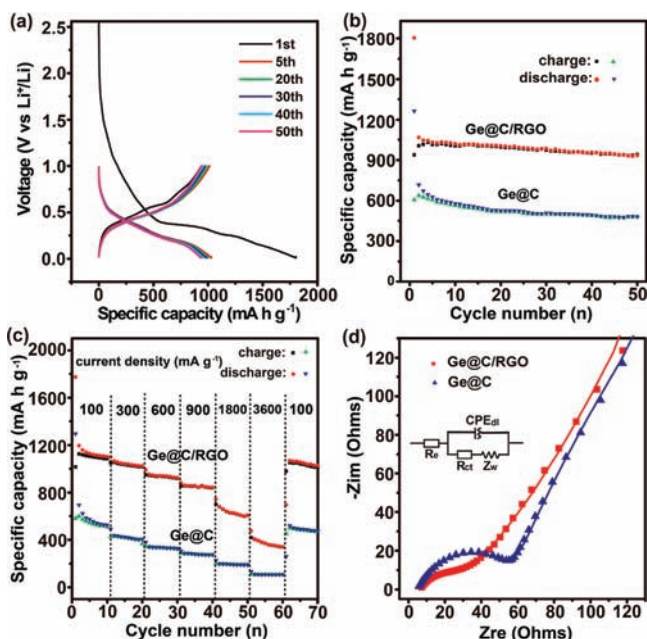
Figure 4. (a) Discharge–charge curves of Ge@C/RGO nanocomposites cycled between 0 and 1.0 V under a current density of 50 \text{ mA g}^{-1} . (b) Cycling behaviors of Ge@C/RGO nanocomposites and Ge@C NPs under a current density of 50 \text{ mA g}^{-1} . (c) Cycling performances of Ge@C/RGO nanocomposites and Ge@C NPs under different current densities. (d) Nyquist plots of the electrodes of Ge@C/RGO nanocomposites and Ge@C NPs.
